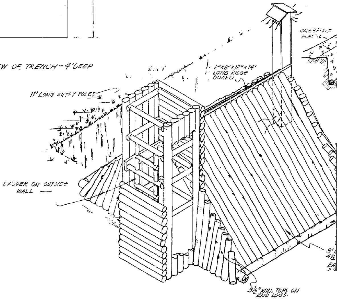
Fig. A-4.1. Two-Family A-Frame Pole Shelter, Semiburied.
